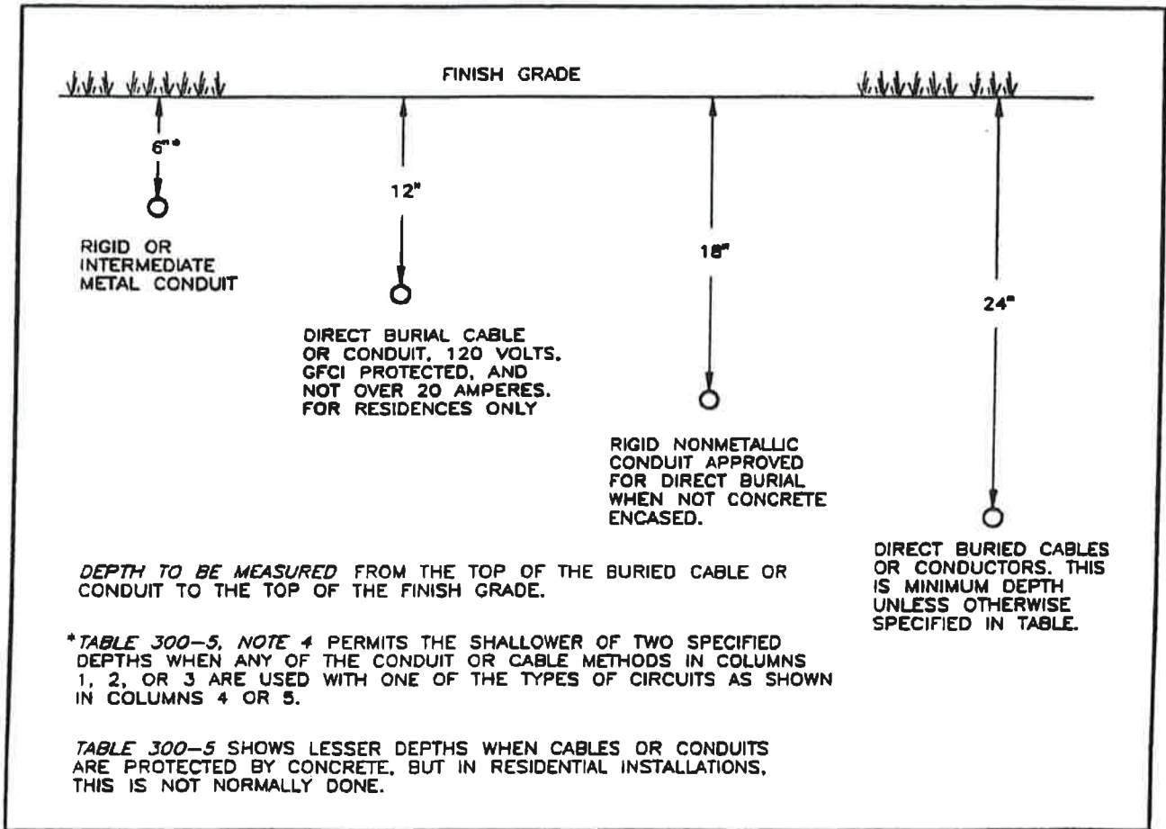
Fig. 16-12C Minimum depths for cables and conduits installed underground.
