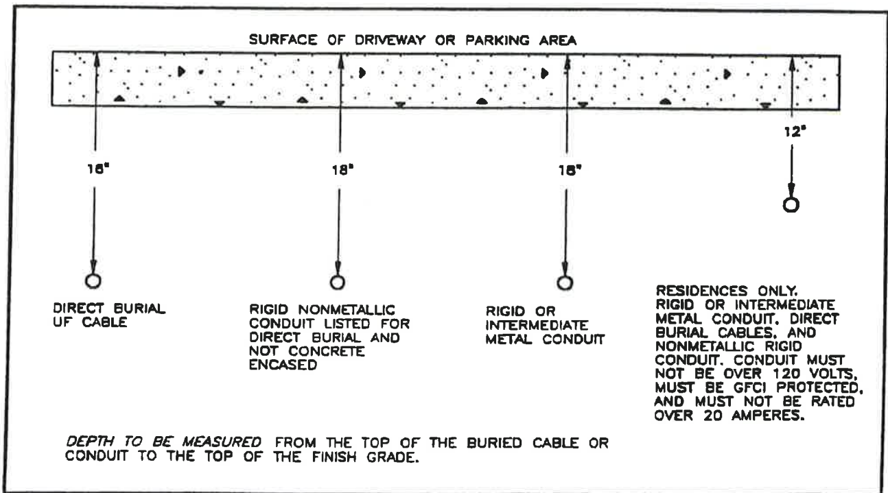
Fig. 16-12D Depth requirements under residential driveways and parking areas. These depths are permitted for one- and two-family residences.
